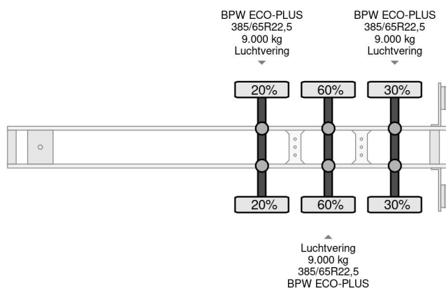
Schmitz Cargobull SKO 24 DOUBLE STOCK CLOSED BOX ...
