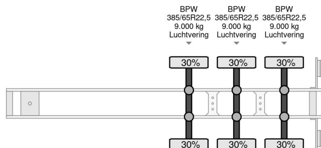
Van Hool 3B1057 3-AXLE 13.60 OPEN TRAILER WITH ALUM...
