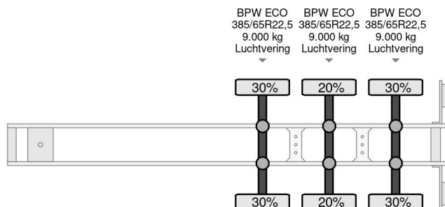
Pacton / JUMBO 3-AXLE CLOSED BOX WITH FULL STEEL ...
