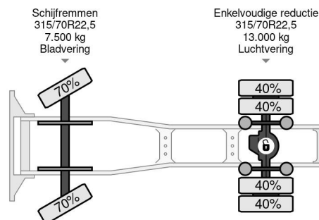
DAF XF 95.480 SPACECAB (EURO 4 / ZF16 MANUAL... 4x2
